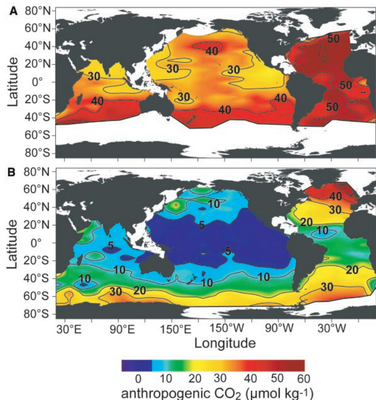
Fig. 4. Maps of anthropogenic \text{CO}_2 on the (A) 26.0 and (B) 27.3 potential density surfaces. Bold lines at the edge of the colored region indicate areas where the density surface outcrops. The highest values are generally observed closest to the outcrop and decrease toward the equator.
