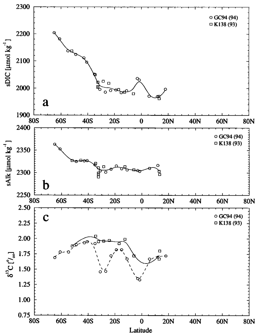
Figure 9. Same as Figure 8, except for the eastern Pacific Ocean (east of 120°W). Shown are the combined results of two cruises which span the period from 1993 to 1994. For \delta^{13}\text{C} (Figure 9c), two spline fits are shown to represent the different trends exhibited by the two different cruises.
