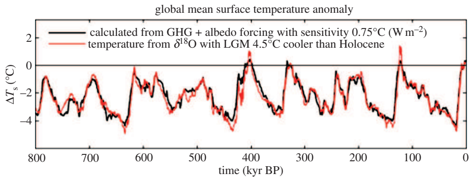
Figure 6. Calculated surface temperature for forcings of figure 5c with a climate sensitivity of 0.75°C per W m -2 , compared with 2 \times \Delta T_{do} . Zero point is the Holocene (10 kyr) mean.
