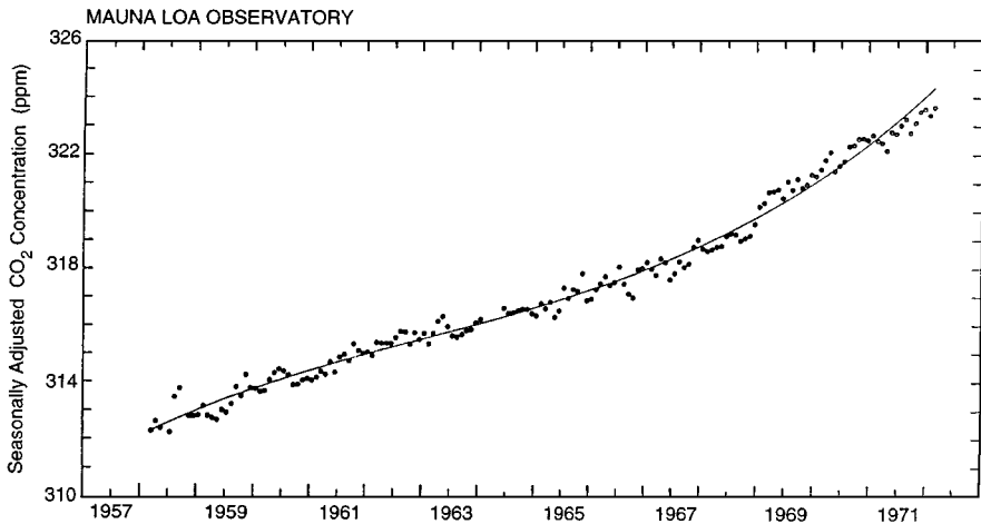
Figure 8 Secular trend of atmospheric CO 2 concentration at Mauna Loa. Circles represent monthly averages, seasonally adjusted by subtracting the 6- and 12-month cyclic terms used in deriving the curve of Figure 7. The rising curve is a cubic secular trend function as in Figure 6. (Source: Ref. 15)
